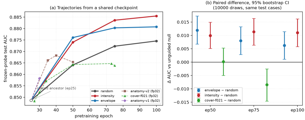
Figure 2: (a) Frozen-probe test AUC against pretraining epoch. All arms fork from the same epoch-25 checkpoint (open circle) and differ only in masking policy. Solid lines are the precision-matched fp16 family; dashed lines are fp32 arms and must not be compared vertically against the solid lines. (b) The actual inference: paired differences against the unguided null on identical test cases, with 10,000-resample bootstrap intervals. All six intervals exclude zero. We plot paired differences rather than per-arm error bars because marginal intervals carry between-case variance that cancels in a paired comparison, and would understate the evidence.
