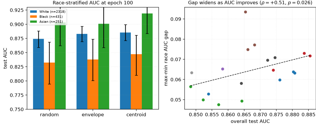
Figure 5: Left: race-stratified AUC at epoch 100. Error bars are 3,000-resample class-stratified percentile bootstrap intervals within each group, with fitted heads fixed and per-group n in the legend; the bars sit on a truncated axis, so bar height exaggerates the differences and only the plotted positions should be read. The black subgroup is lowest under every policy, yet every group point estimate rises from RANDOM to CENTROID. Right: max–min race gap against aggregate AUC, one point per probe over the 19 probes that carry a race summary. The dashed line is a least-squares fit while the quoted correlation is Spearman. The slope is positive but fails multiplicity correction at checkpoint level and does not survive branch-level aggregation (Table 6), so we draw no trend conclusion from it.
