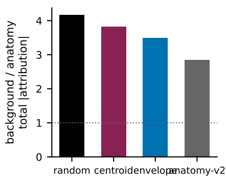
(c) Background carries most of the total attribution mass
