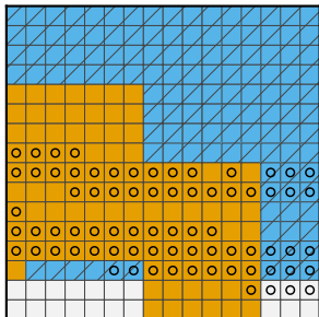
(c) V2: scored / sampled indices
