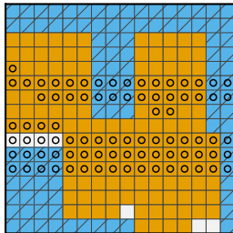
(c) Envelope
