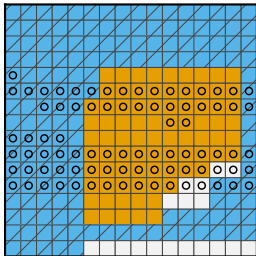
(a) Random
