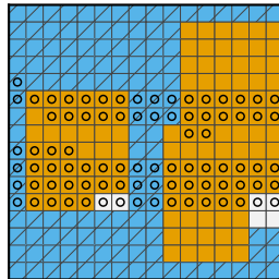
(e) COVER
