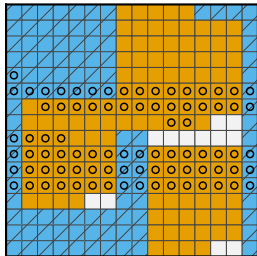
(b) Centroid
