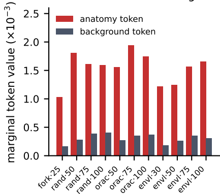
(a) Anatomy tokens are worth 3.9--6.6 \times more than background
