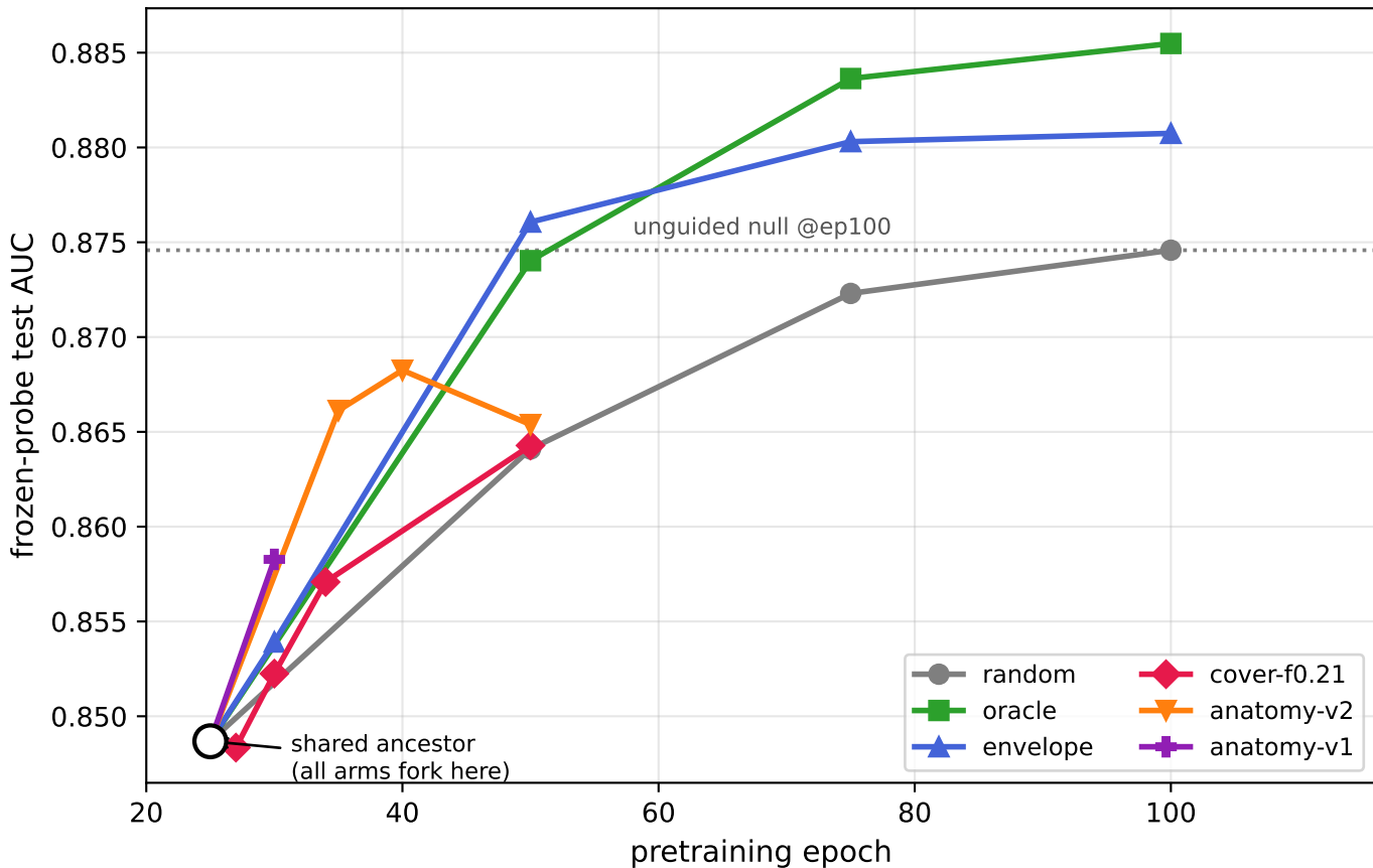
Downstream AUC by masking policy all arms share one ancestor checkpoint and one probe protocol
