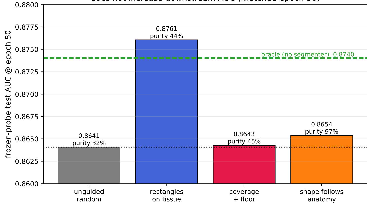
Increasing anatomical specificity of the mask (left to right) does not increase downstream AUC (matched epoch 50)
