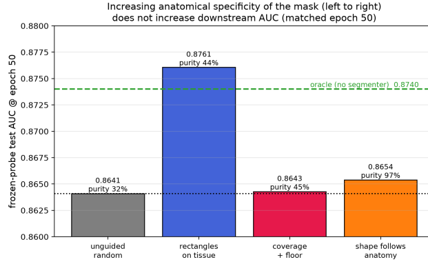
Figure 6: The matched-epoch-50 result arranged as a ladder of increasing anatomical specificity. Companion to Figure 3.
