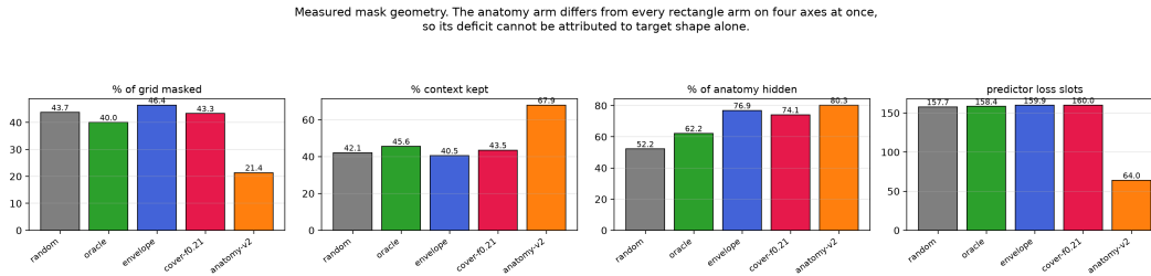
Figure 7: Measured mask geometry per policy, 600 held-out slices. The four rectangle policies are closely matched on every axis, so their comparison is near single-variable. The anatomy policy diverges on all four simultaneously — half the masking ratio, 1.6\times the context, 0.4\times the predictor loss slots — which is why we decline to attribute its deficit to target shape.
