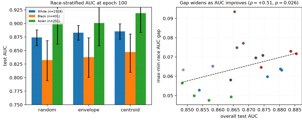
Figure 5: Left: race-stratified AUC at epoch 100. Error bars are 10,000-resample percentile bootstrap intervals over test volumes, with the per-group n in the legend; the bars sit on a truncated axis, so bar height exaggerates the differences and only the plotted positions should be read. The black subgroup is lowest under every policy, yet every group improves from RANDOM to CENTROID. Right: max-min race gap against aggregate AUC, one point per probe over the 19 probes that carry a race summary. The dashed line is a least-squares fit while the quoted correlation is Spearman. The slope is positive and passes multiplicity correction at checkpoint level, but does not survive branch-level aggregation (Table 6), so we draw no trend conclusion from it.
