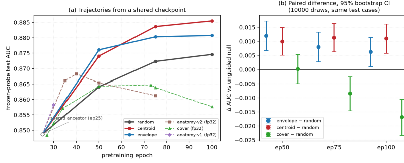
Figure 2: (a) Frozen-probe test AUC against pretraining epoch; note the truncated AUC axis. All arms fork from the same epoch-25 checkpoint (open circle). Solid lines are the precision-matched fp16 family; dashed lines are fp32 arms and must not be compared vertically against the solid lines. (b) The actual inference: paired differences against the unguided null on identical test cases, 10,000-resample percentile bootstrap intervals. Every ENVELOPE and CENTROID interval excludes zero; COVER straddles zero at epoch 50 and is negative thereafter. Paired differences replace per-arm error bars: marginal intervals carry between-case variance that cancels in a pairing and would understate the evidence.
