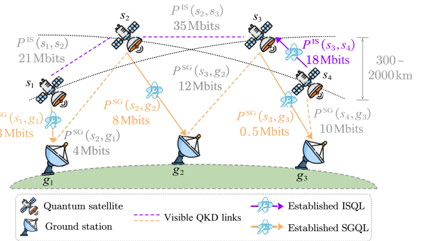
Fig. 5. Illustration of the MinRKV-based QKD link establishment scheme.
