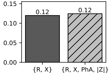
Bootstrap 95% CI width for \Delta R^2
