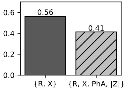
True-signal feature selection rate
