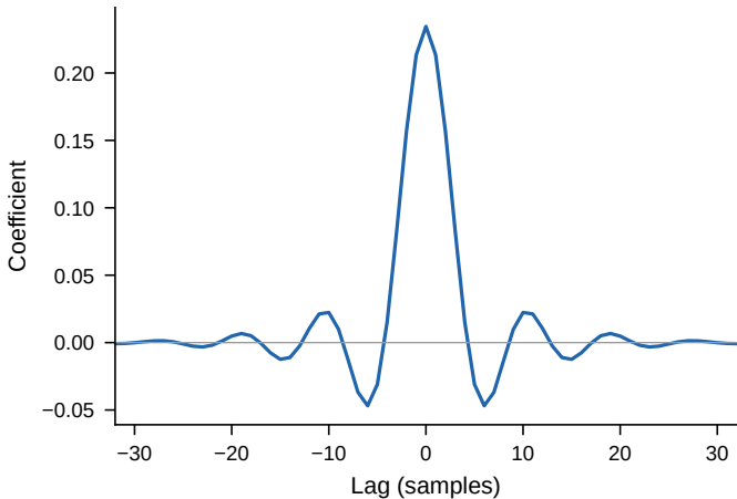
65-tap symmetric impulse response
