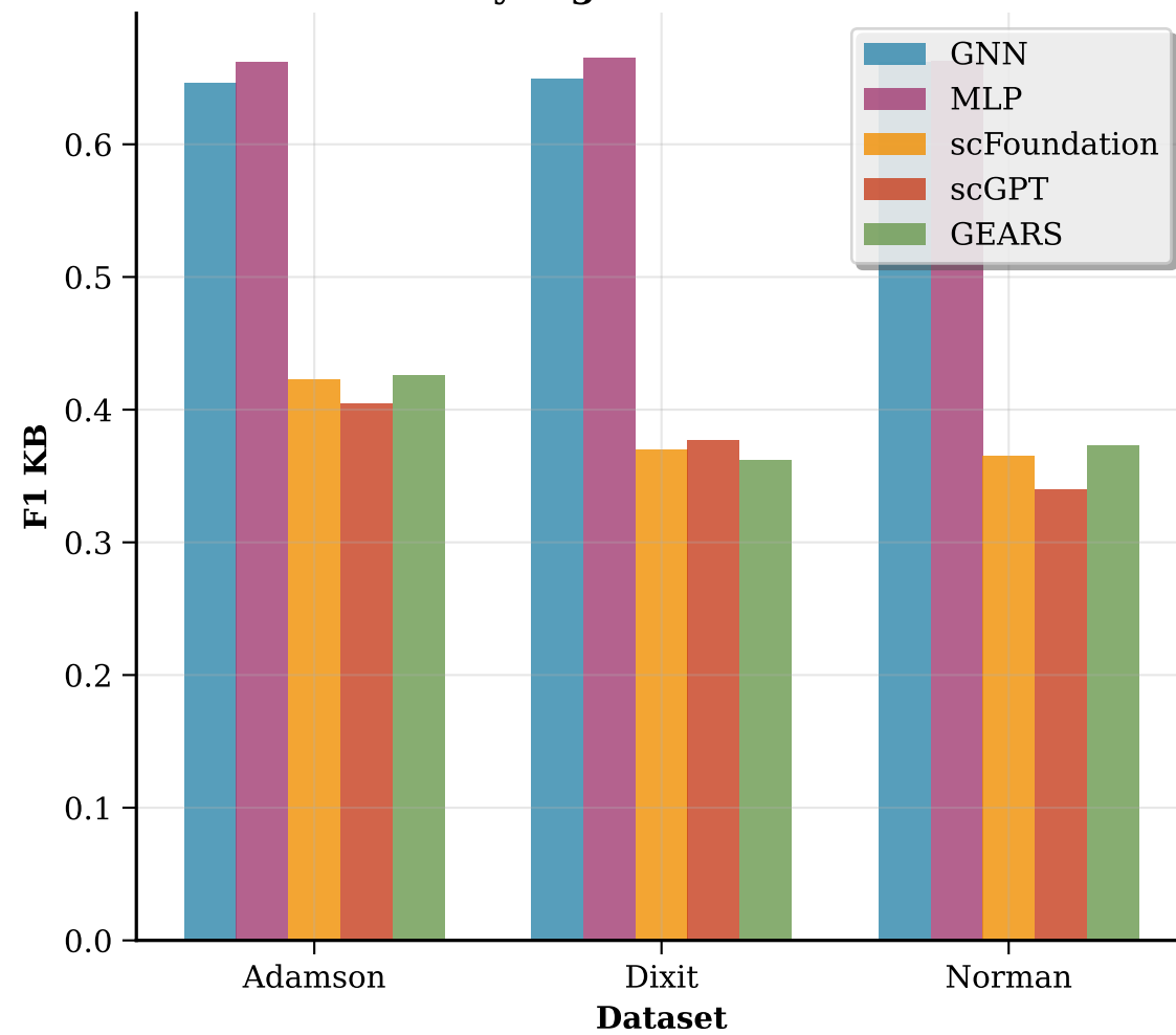
F1 KB by Algorithm and Dataset
