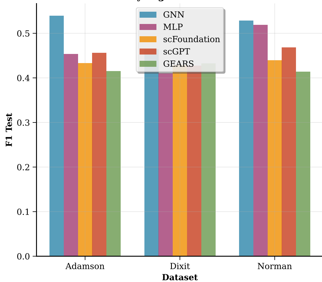
F1 Test by Algorithm and Dataset
