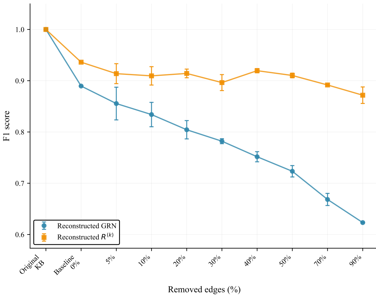
Reconstruction accuracy
