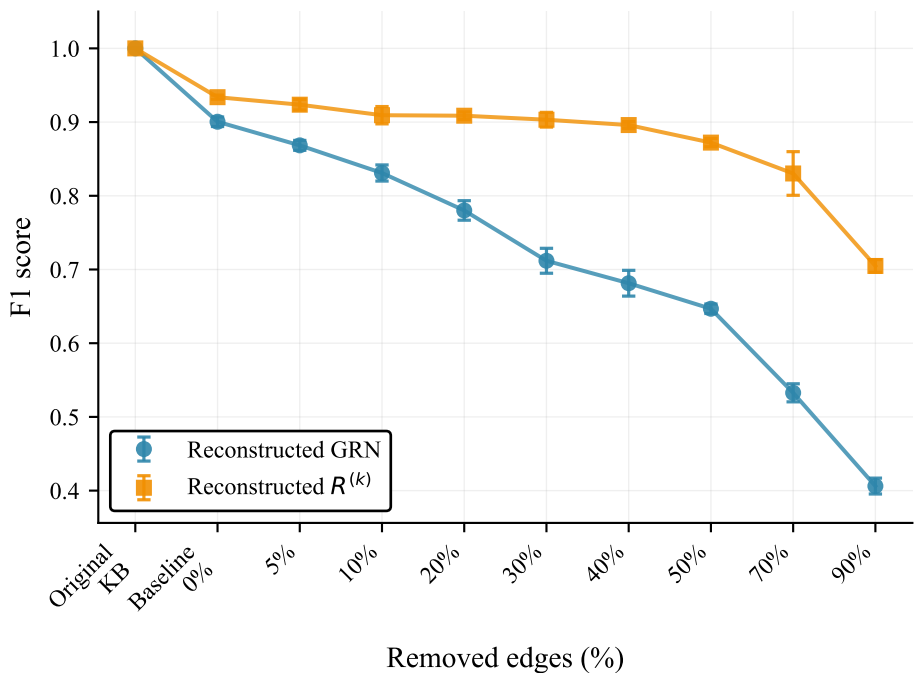
Reconstruction accuracy
