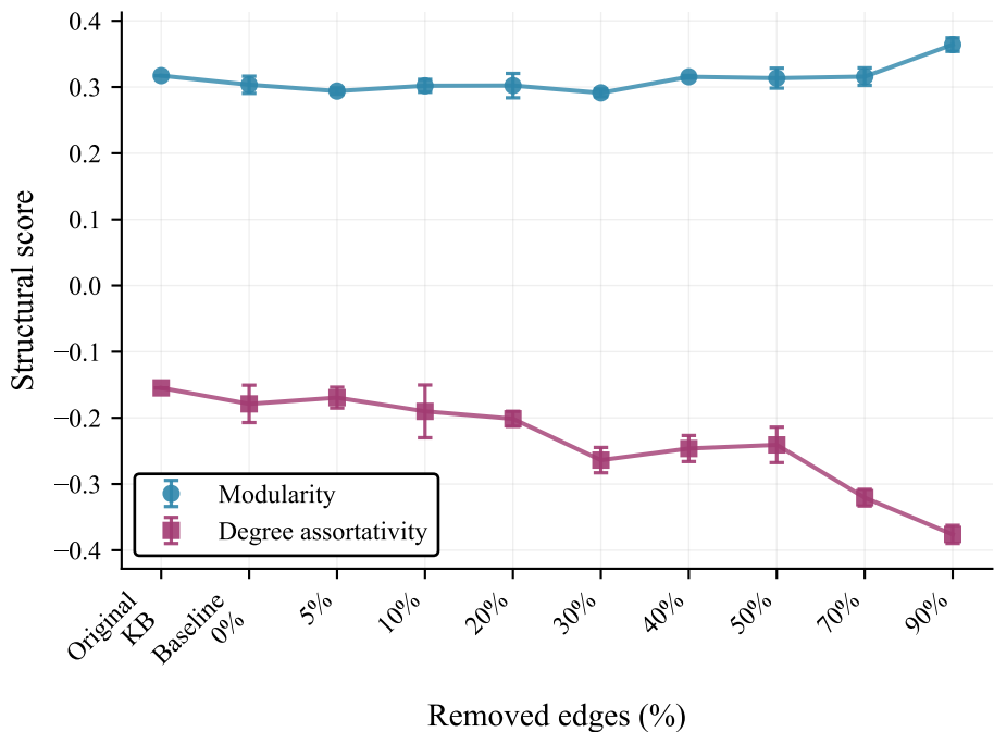
Structural properties of reconstructed networks
