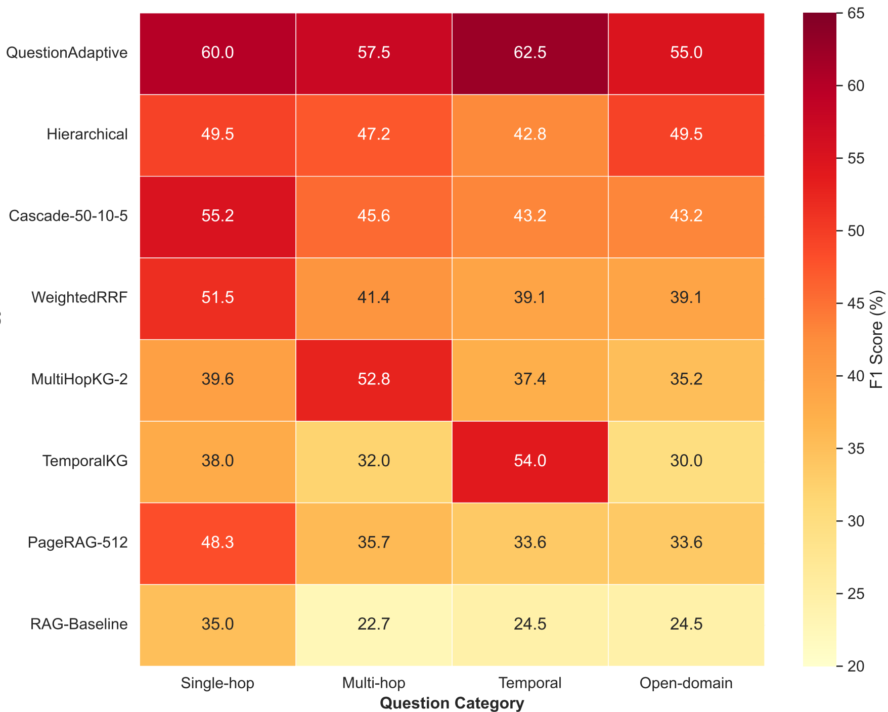
MemSt Performance by Question Category
