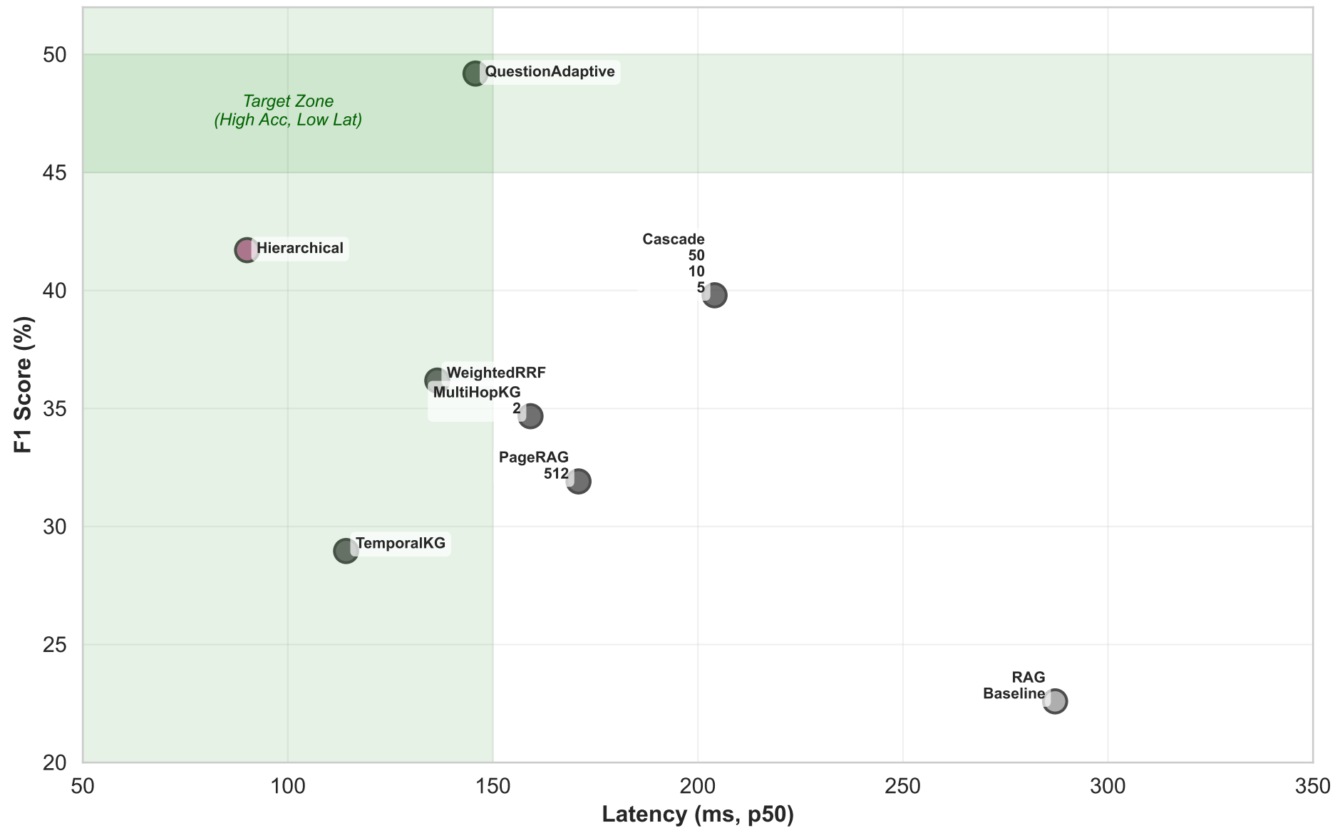
Accuracy vs Latency Tradeoff (Bubble size = Token count)
