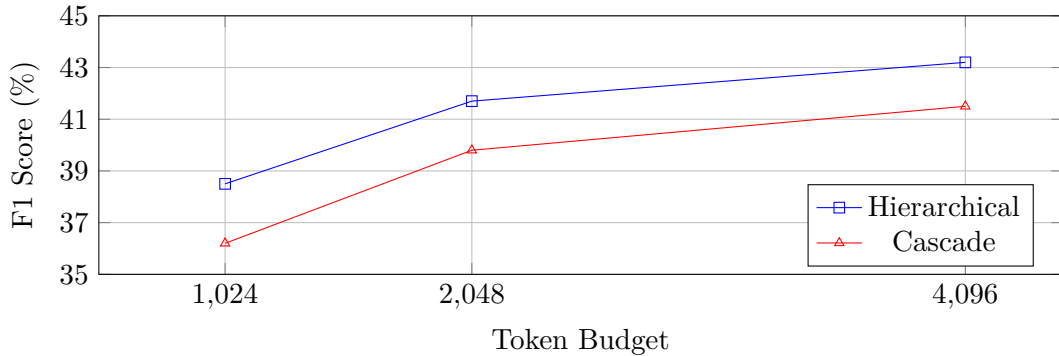
Figure 2: Effect of token budget on F1 score. Diminishing returns beyond 2,048 tokens.
