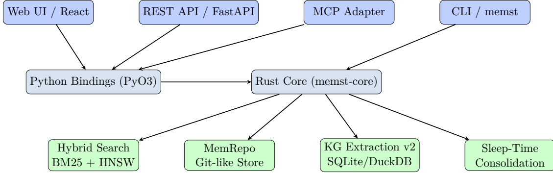
Figure 1: MemSt architecture overview showing the multi-layer design with interfaces (top), language bindings (middle), and core storage/processing components (bottom).
