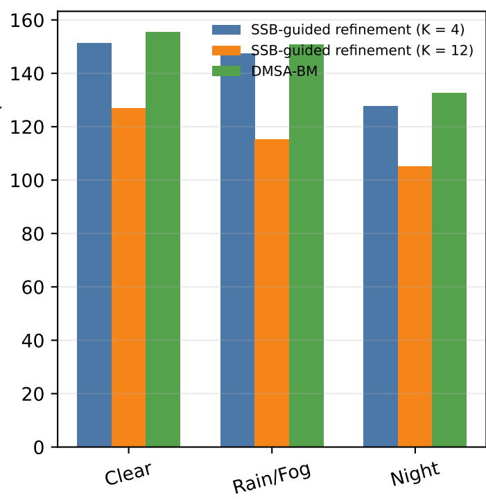
Mean effective user rate (Mbps)
