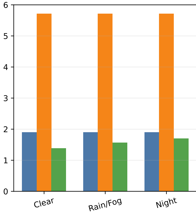
CSI-RS overhead (%)
