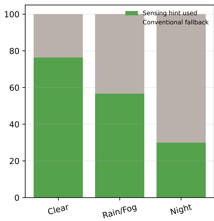
CSI-event fraction (%)
