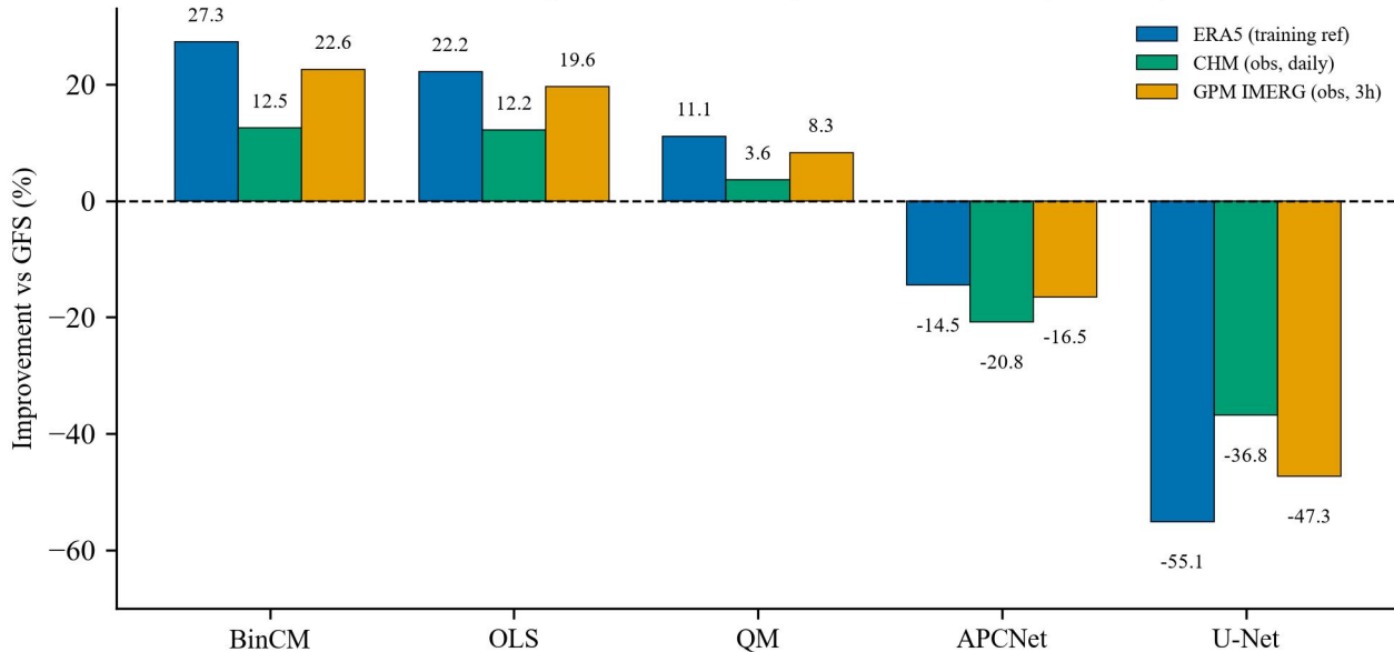
Consistent ranking: BinCM > OLS > QM > GFS > APCNet (3-h scales)
