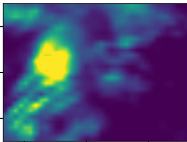
GFS (raw) (3.47)
