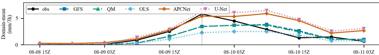
GPM IMERG (obs) (5.83)
