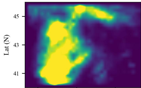
GPM IMERG (obs) (5.83)
