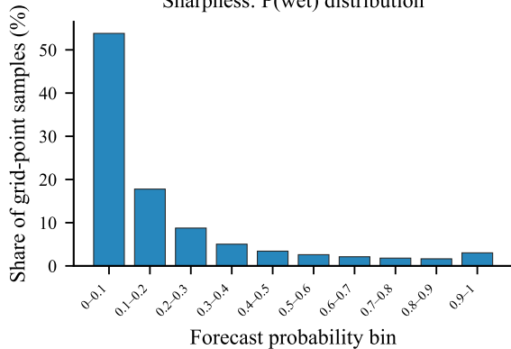
Sharpness: P(wet) distribution
