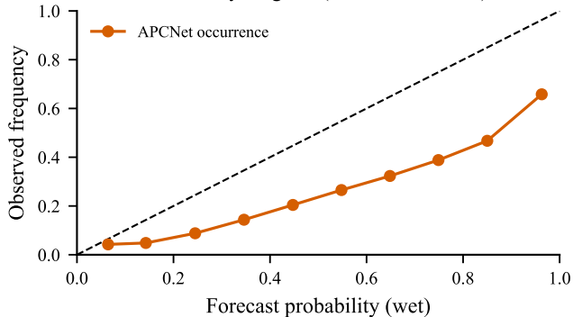
Reliability diagram (0.1 mm threshold)
