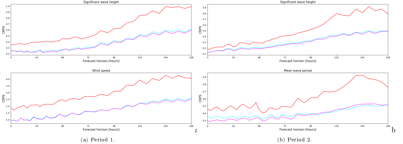
Figure 12: Variation of CRPS with forecast horizon for (a) out-of-sample Period 1 (1 September 2023 - 30 April 2024) and (b) out-of-sample Period 2 (1 September 2024 - 31 December 2024) for the uncalibrated deterministic forecast (red), the forecast calibrated using LR (cyan) and the forecast calibrated using NHGR (magenta).
