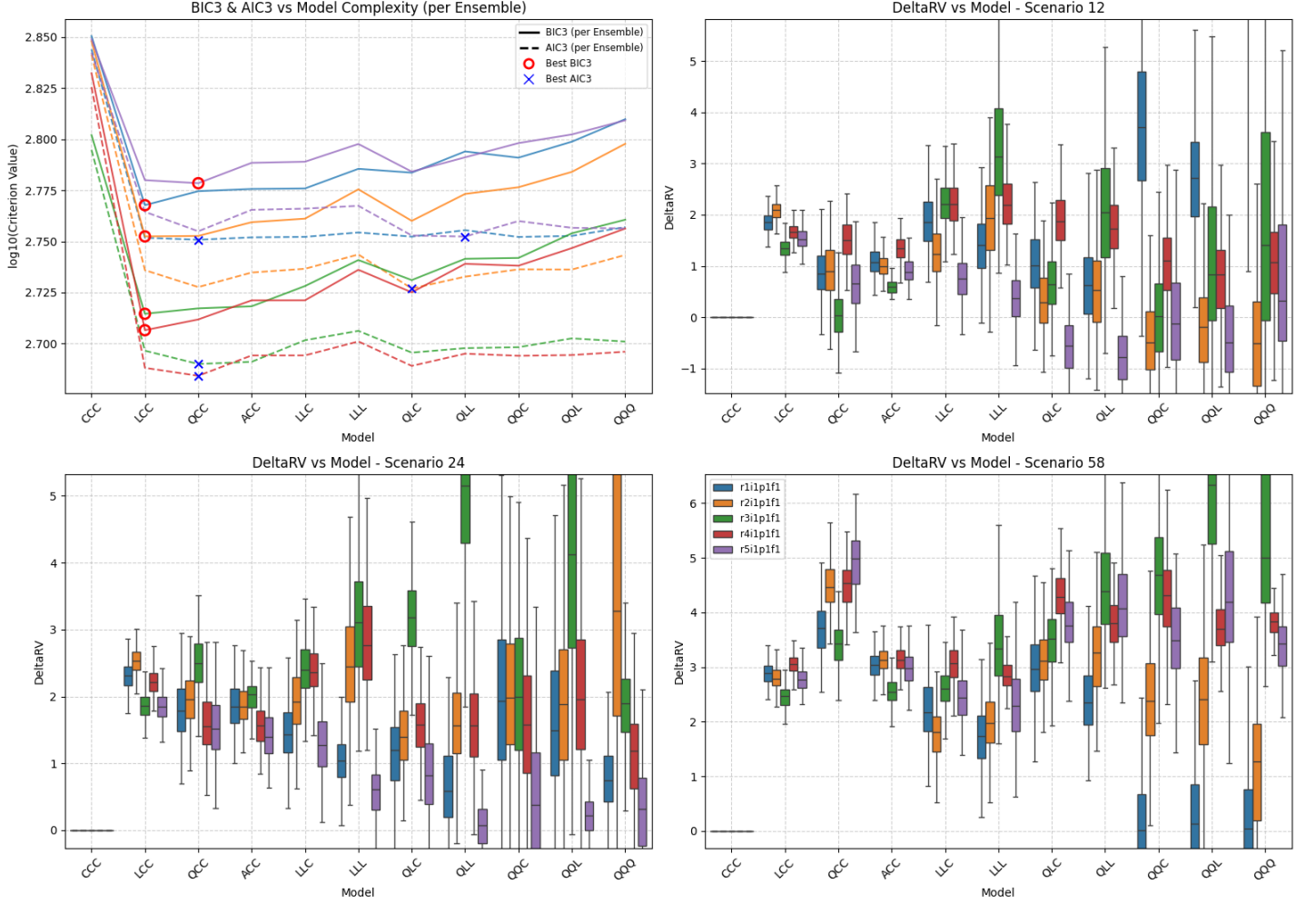
Figure SM2: Summary of scenario-coupled GEV regression for regional annual maxima of the Antarctic region using ACCESS-CM2 GCM data. Top left: plots of BIC3 (solid line) and AIC3 (dashed line) for each available ensemble (distinguished by colour, see Table 2 of the main text and legend in bottom-right panel); optimal model choice using BIC3 (AIC3) indicated using red disc (blue cross). Top right: box-whisker plots summarising the distribution of the difference in the 100-year return value between 2025 and 2125 ( \Delta Q_1 ; see Equation 7) for climate scenario SSP126 as a function of fitted model complexity (x-axis) and ensemble (distinguished by colour, with consistent ensemble colouring across panels); location of horizontal centre line of each box indicates posterior median of \Delta Q_1 ; location of top (bottom) side of each box indicates 75%ile (25%ile) point, and top (bottom) of whiskers the 97.5%ile (2.5%ile) point of the posterior distribution. Bottom left and right: analogues of top right for scenarios SSP245 ( \Delta Q_2 ) and SSP585 ( \Delta Q_3 ). Value of \Delta Q_j , j = 1, 2, 3 under model CCC is identically zero, and is omitted from bottom panels when convenient to provide better illustration of the variation in estimates under more complex models. For comparison with Figure 6 of the main text.
