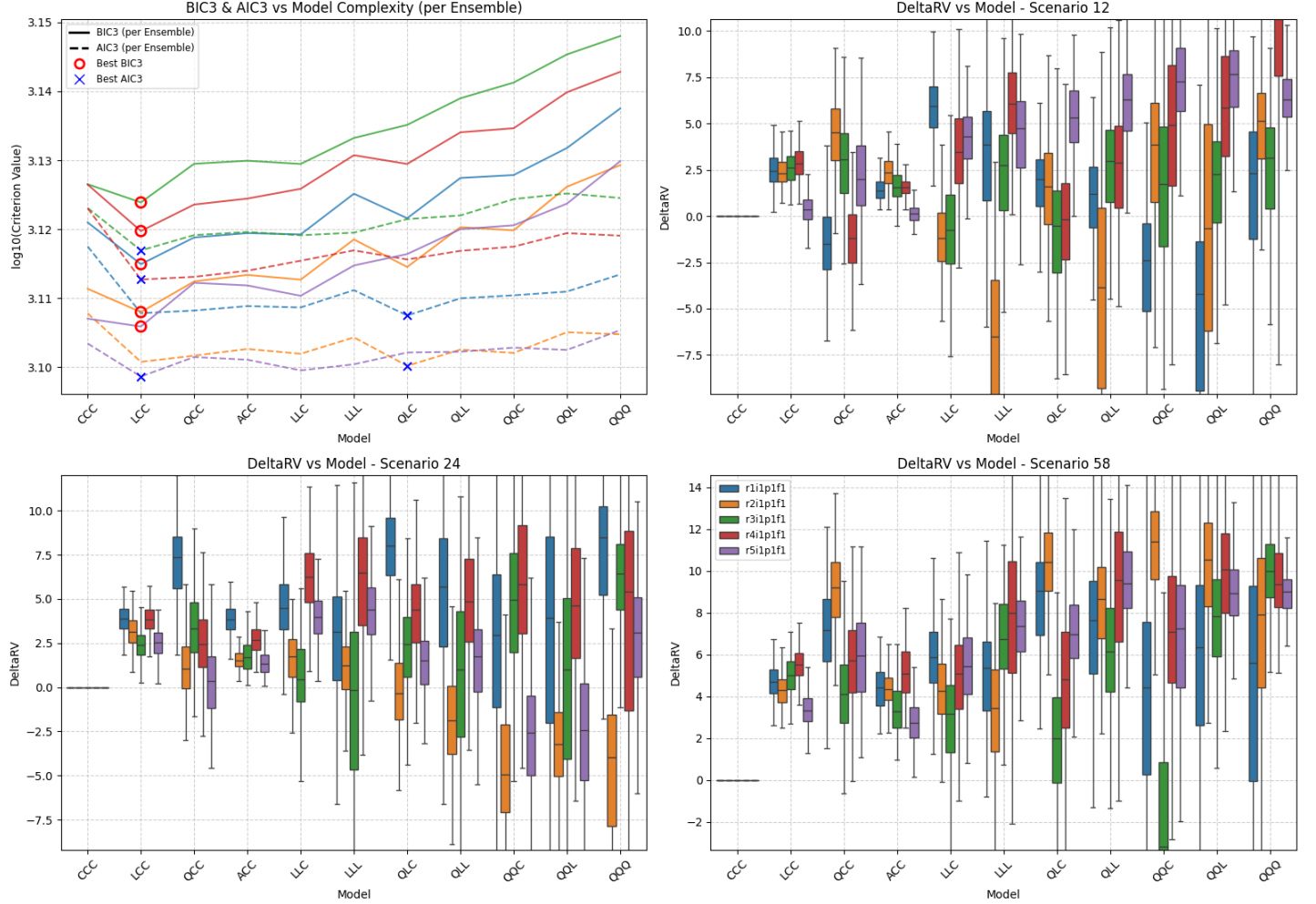
Figure SM41: Summary of scenario-coupled GEV regression for regional annual minima of the Dasht-e Lut region using ACCESS-CM2 GCM data. Top left: plots of BIC3 (solid line) and AIC3 (dashed line) for each available ensemble (distinguished by colour, see Table 2 of the main text and legend in bottom-right panel); optimal model choice using BIC3 (AIC3) indicated using red disc (blue cross). Top right: box-whisker plots summarising the distribution of the difference in the 100-year return value between 2025 and 2125 ( \Delta Q_1 ; see Equation 7) for climate scenario SSP126 as a function of fitted model complexity (x-axis) and ensemble (distinguished by colour, with consistent ensemble colouring across panels); location of horizontal centre line of each box indicates posterior median of \Delta Q_1 ; location of top (bottom) side of each box indicates 75%ile (25%ile) point, and top (bottom) of whiskers the 97.5%ile (2.5%ile) point of the posterior distribution. Bottom left and right: analogues of top right for scenarios SSP245 ( \Delta Q_2 ) and SSP585 ( \Delta Q_3 ). Value of \Delta Q_j , j = 1, 2, 3 under model CCC is identically zero, and is omitted from bottom panels when convenient to provide better illustration of the variation in estimates under more complex models. For comparison with Figure 6 of the main text.
