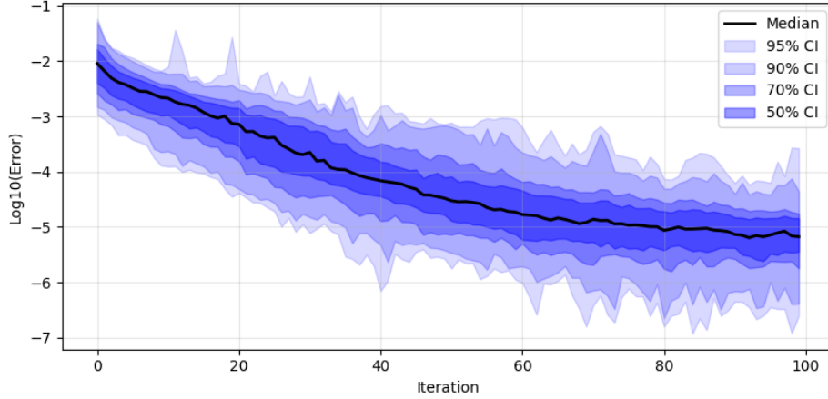
Figure 15: Distribution of log-scale absolute error \Delta_{\text{GP}} in the GP probability estimate with respect to iteration, trained using U^{(1)} with \lambda = \lambda^* . The trend in median error is indicated in black, with various confidence intervals shown in blue.
