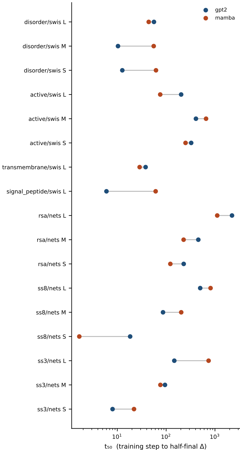
emergence half-time: gpt2 vs mamba
