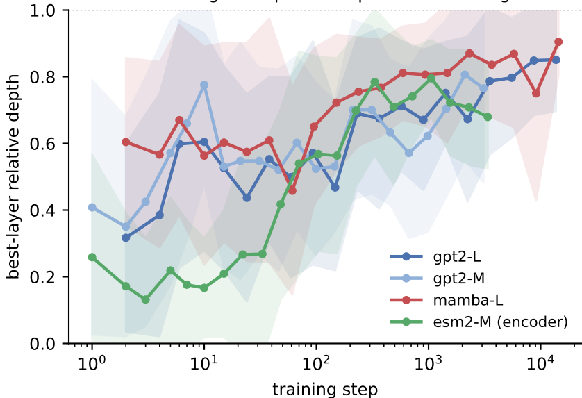
Decoding is deep and deepens over training
