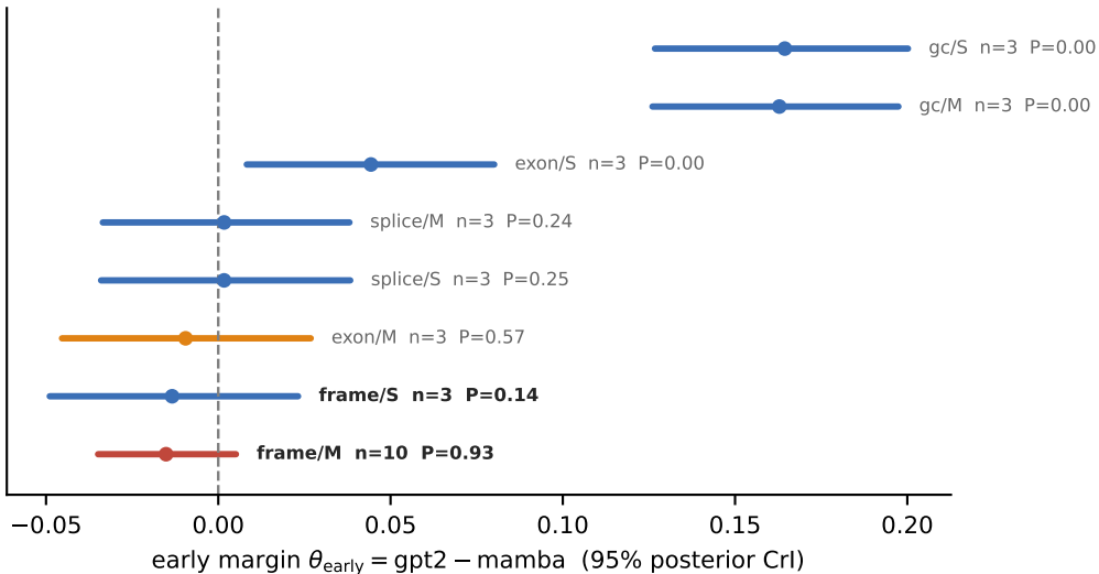
GENOME: hierarchical reversal posterior (partial pooling, 3–10 seeds/cell; red P \geq 0.9 , orange \geq 0.5 , blue < 0.5 )
