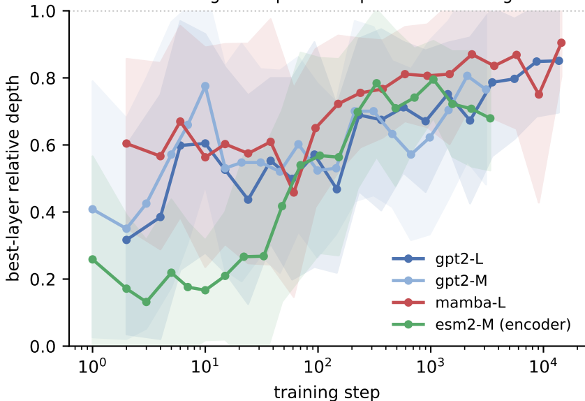
Decoding is deep and deepens over training
