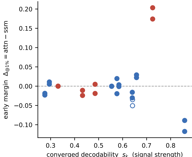
strength alone does NOT predict reversal ( r=+0.03 )
