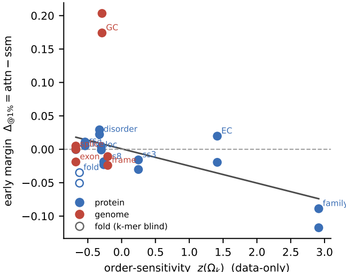
reversal tracks sequential structure r=-0.41 (p=0.041), excl. fold r=-0.46
