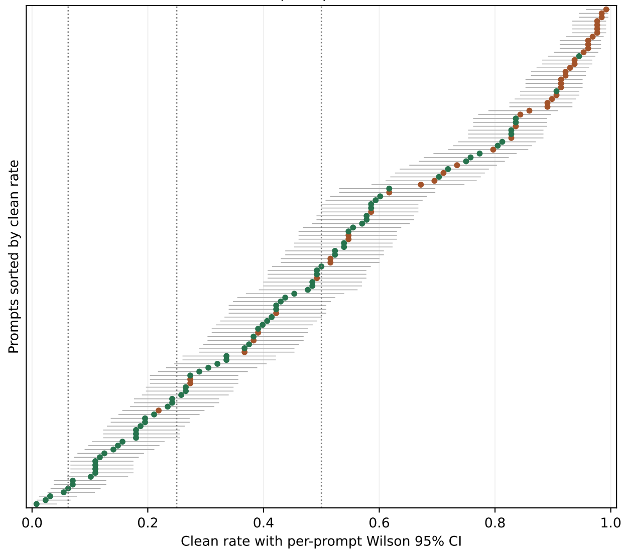
N2 prompt forest
