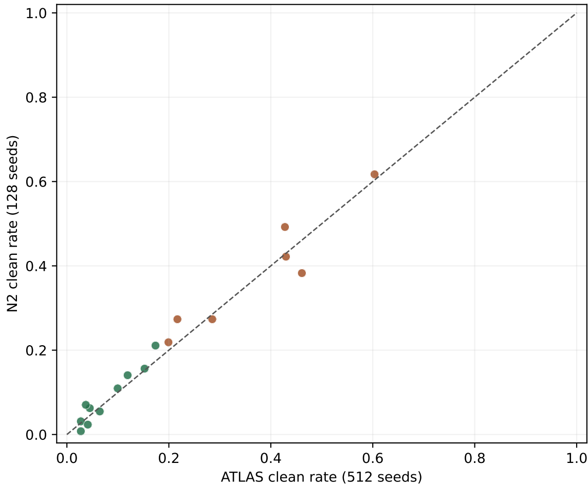
ATLAS to N2 replication (17 overlapping prompts, r=0.983 )
