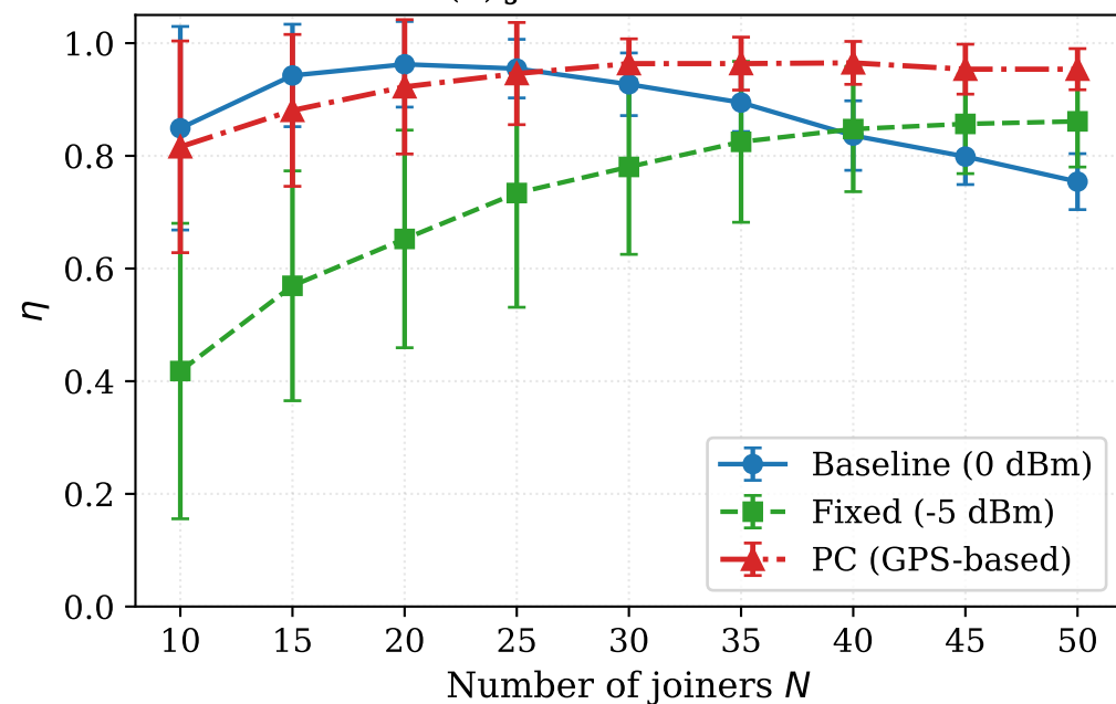
(b) Join success rate
