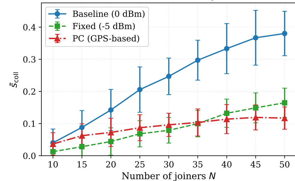
(c) Collision severity
