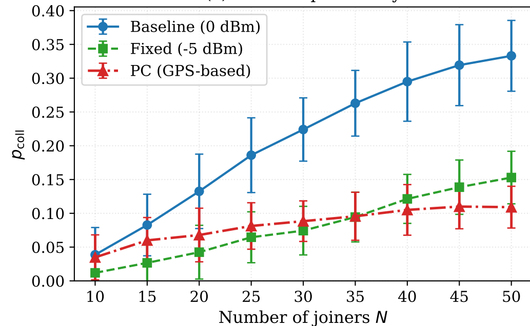
(a) Collision probability
