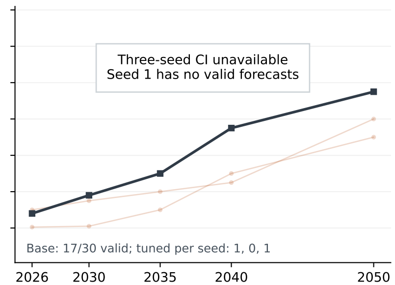
Qwen3-8B-Base
