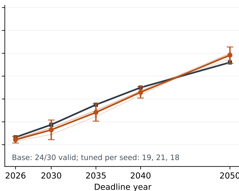
Qwen2.5-72B
