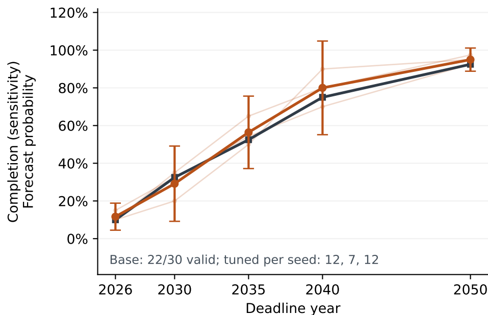
Qwen2.5-7B
