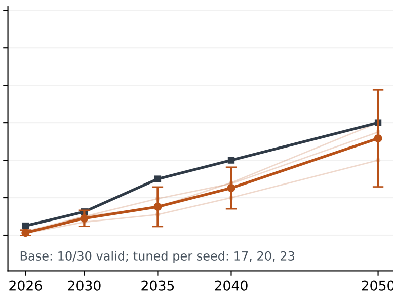
Qwen2.5-72B
