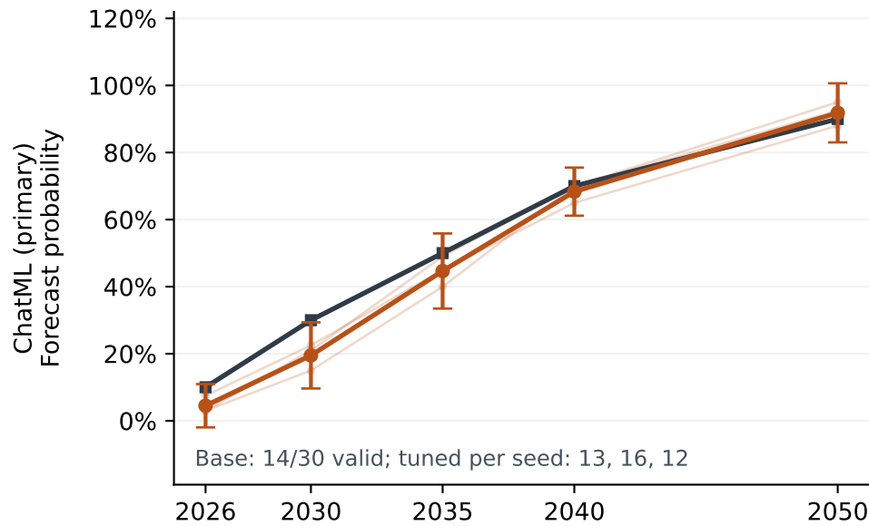
Qwen2.5-7B
