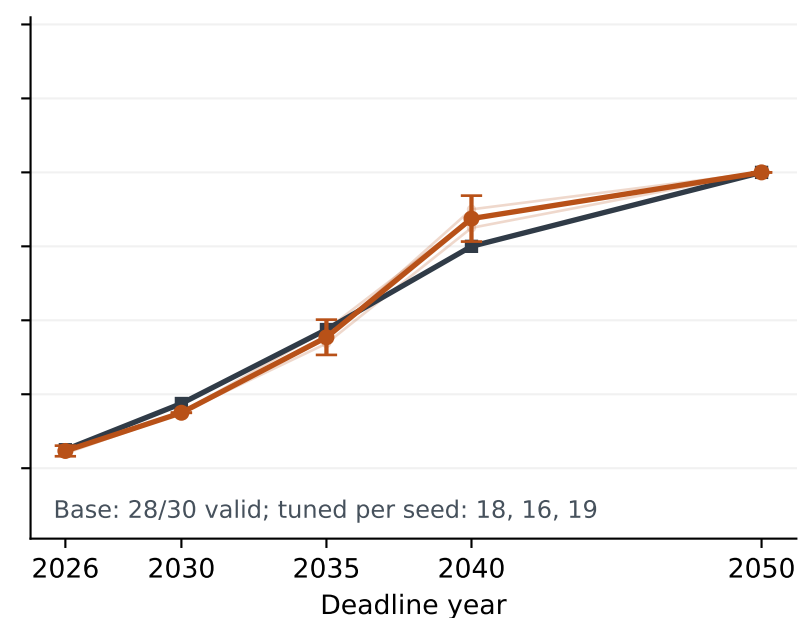
Qwen3-8B-Base
