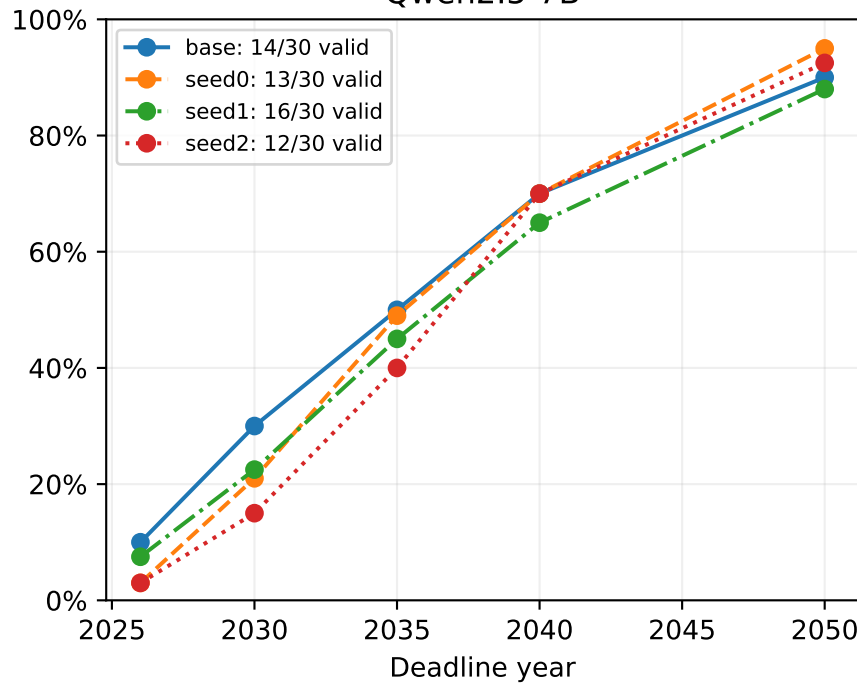
Qwen2.5-7B
