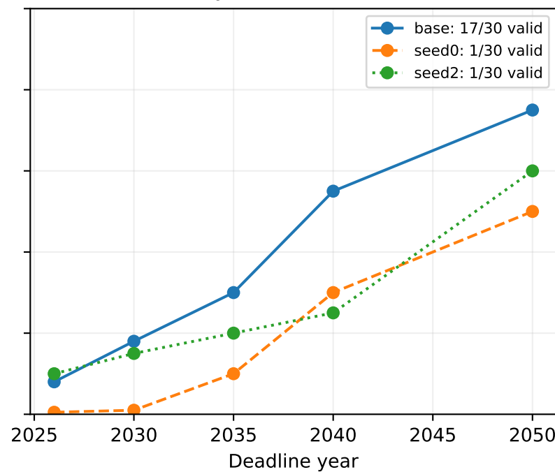
Qwen3-8B-Base
