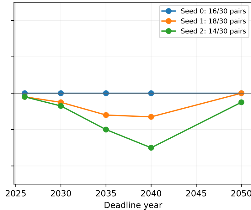
Qwen2.5-72B
