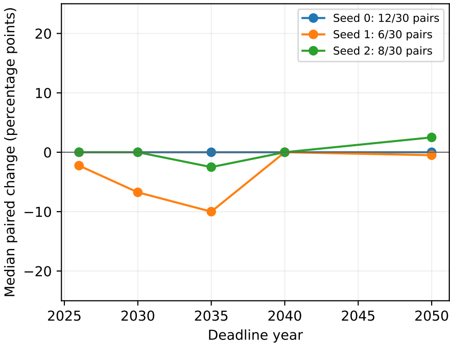
Qwen2.5-7B
