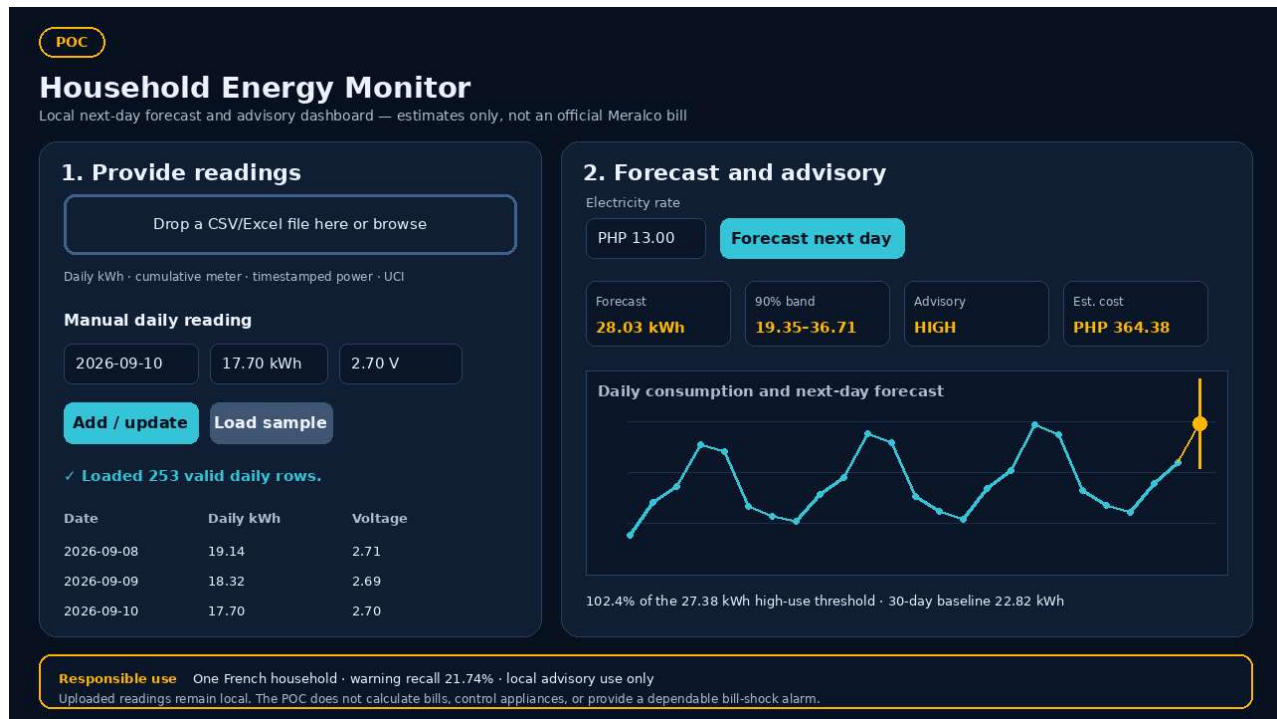
Figure 5. Final Dockerized Dash proof-of-concept dashboard using the included demonstration data.
