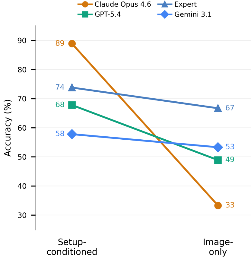
Figure 5: Rank reversal between evaluation conditions. With setup text (left), Claude leads; without setup text (right), the expert leads and Claude drops to the lowest accuracy among all evaluators.
