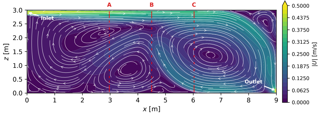
Figure 2: Solver validation against Nielsen et al. (1978) benchmark (9 m \times 3 m, Re \approx 5,000 ). Colour contours show velocity magnitude; white streamlines show the ceiling jet, recirculation zone, and corner vortex. Red markers (A, B, C) indicate the three LDA measurement stations compared in Table 1.
