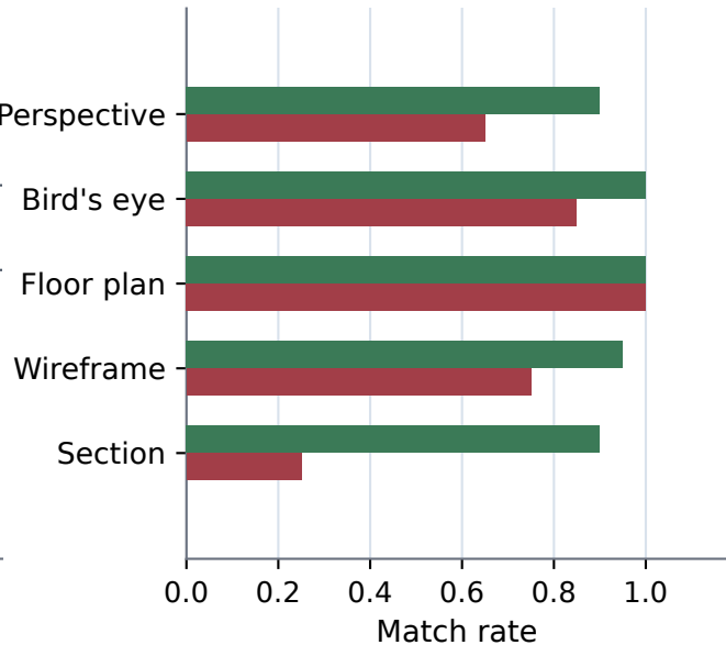
(b) Agreement rates
