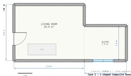
Case 2: L-shaped composite
