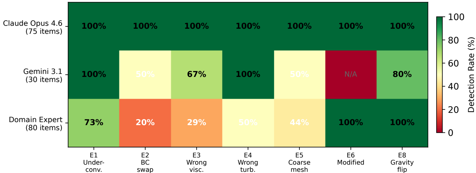
Error Detection Rate by Error Type and Evaluator
