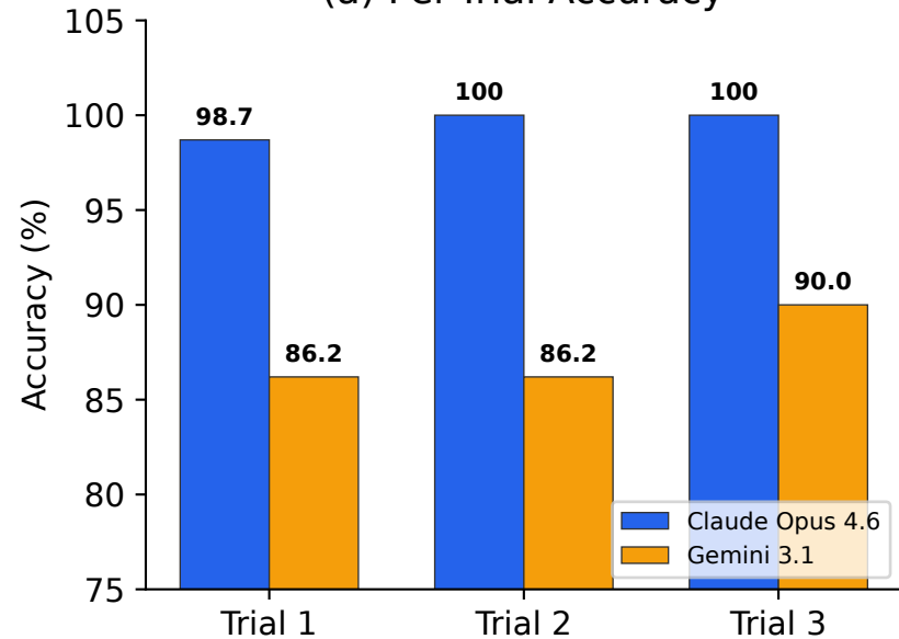
(a) Per-Trial Accuracy
