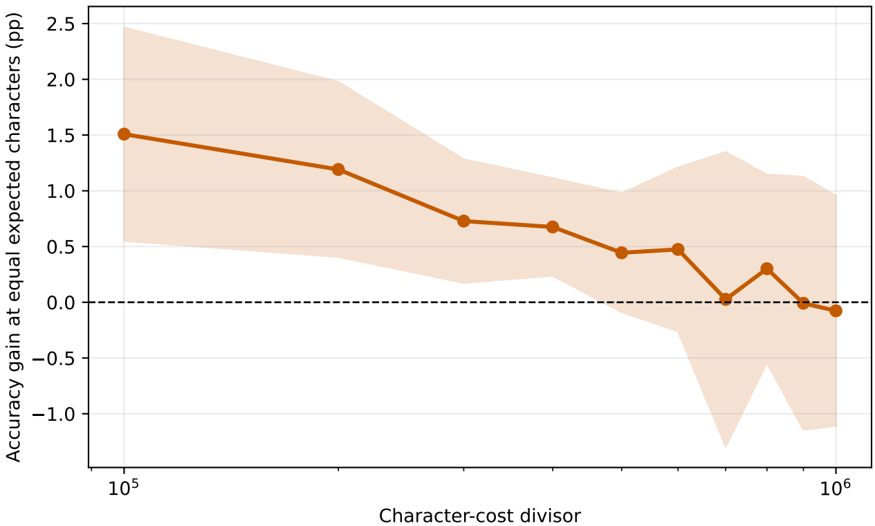
Coding equal-budget accuracy: retained exp-tail selector
