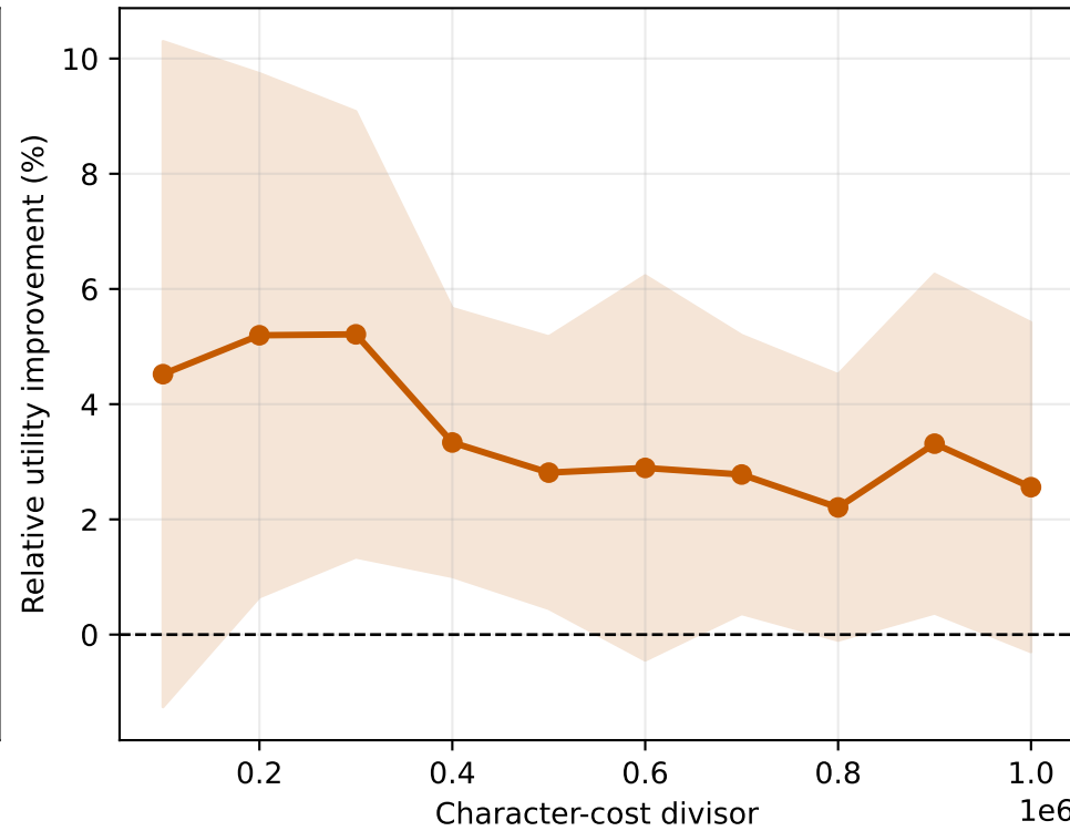
C. Train-selected fixed character budget
