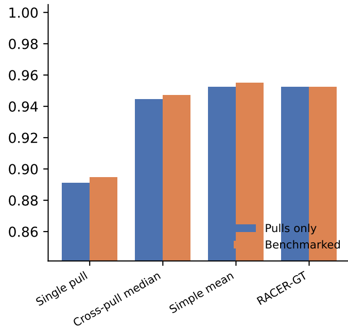
Top-5% peak recall
