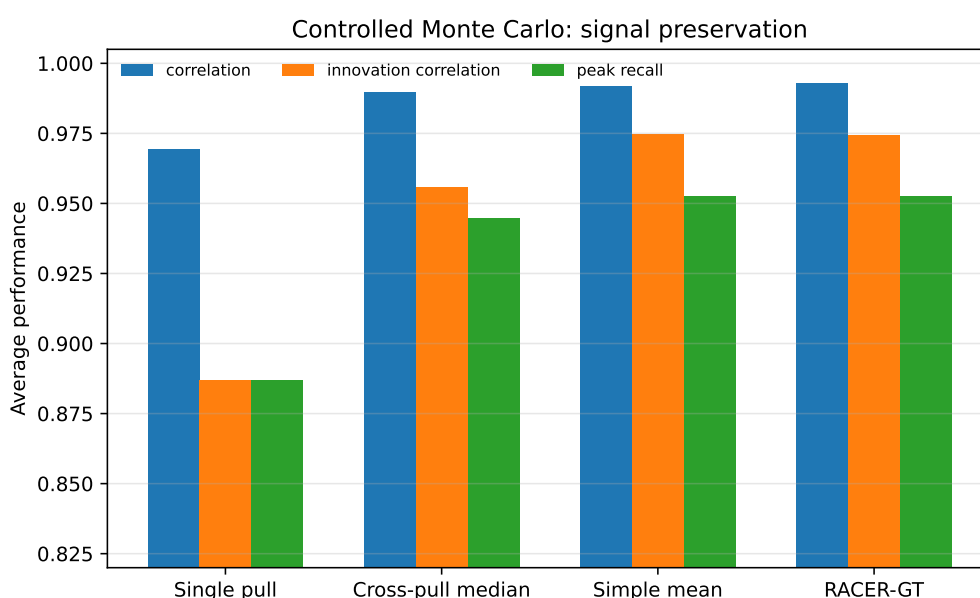
Figure 3: Level correlation、innovation correlation 與 top-5% peak recall。
