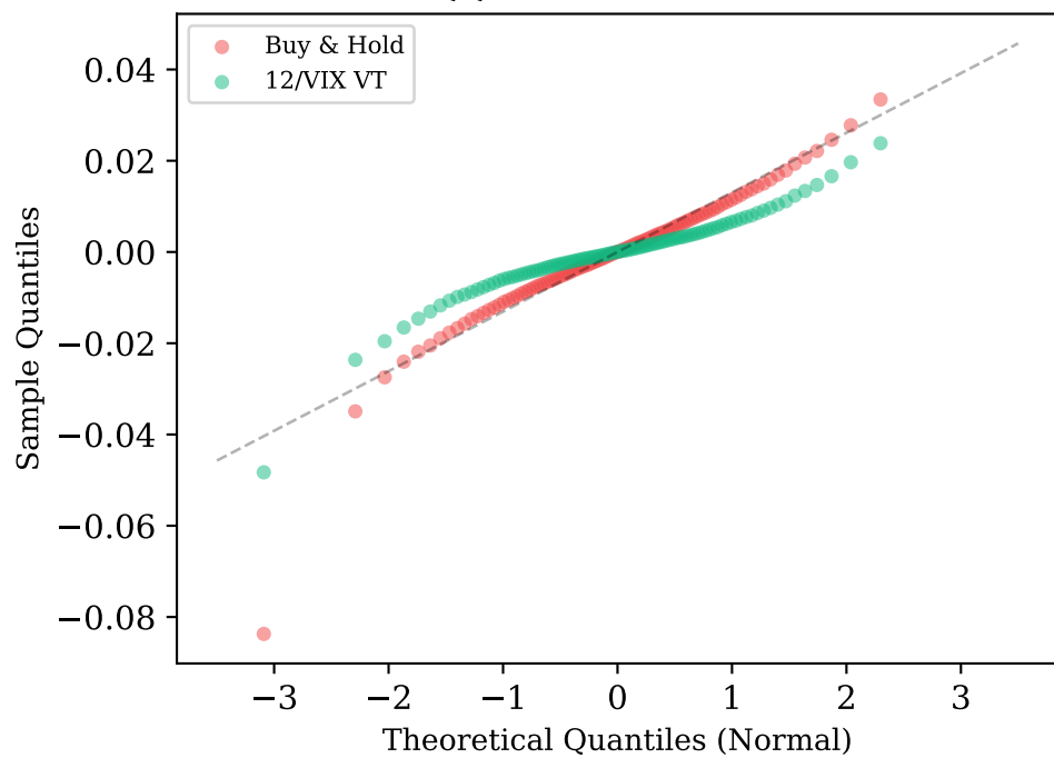
QQ Plot: Tail Behavior
