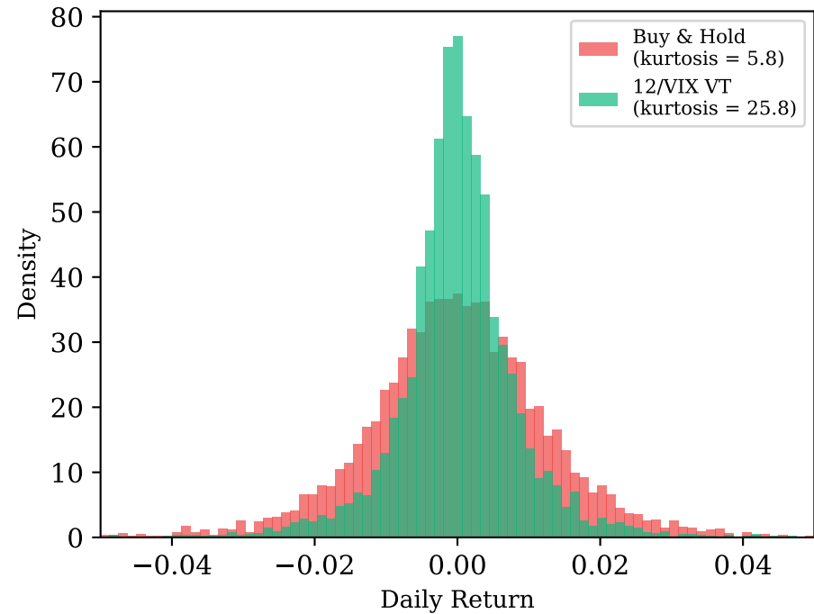
Return Distribution: BH vs VT
